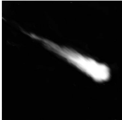
Cometa Halley.
